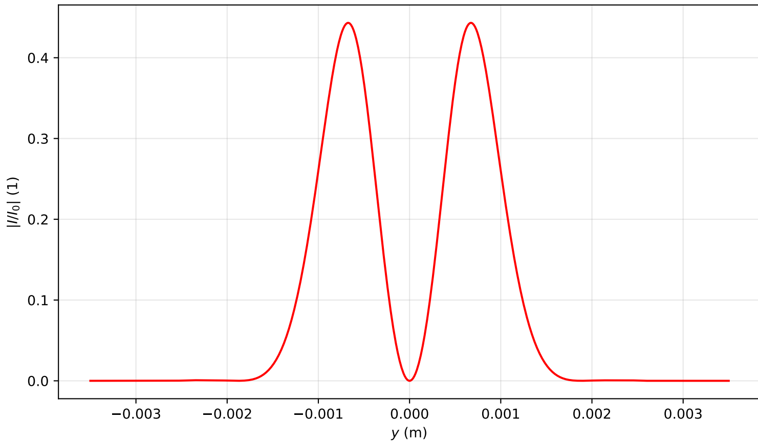
Intensity profile I(x=0, y, z=1.990)/I_0 , \text{Pin}=2.0\text{Pcr} , artificial time
